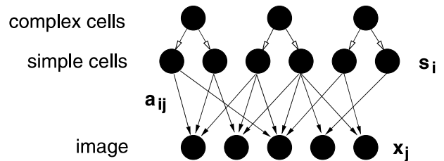
Fig. 2. The extended sparse coding model (Hyvärinen & Hoyer, 2000; Hyvärinen et al., 2001). Each complex cell determines the variance of a group of simple cells.
