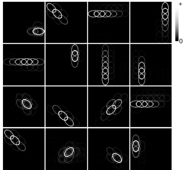
Fig. 7. A representative set of basis functions from the learned basis. The majority of units code the simultaneous activation of collinear complex cells, indicating a smooth contour in the image.
