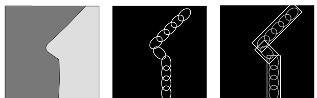
Fig. 8. Contour coding in the model. A hypothetical contour in an image (left) is transformed into complex cell responses (middle). These responses can be sparsely represented using only three higher-order units (right) of the types shown in Fig. 7.
