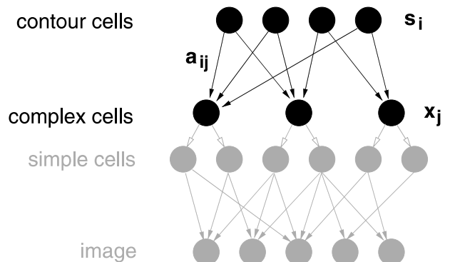
Fig. 3. The simplified hierarchical model investigated in this paper. Model complex cell responses are calculated in a feedforward manner, and these responses are subsequently analyzed by a higher-order sparse coding layer in the network. To emphasize that the lower layers are fixed and not learned, these layers have been grayed out in the figure.
