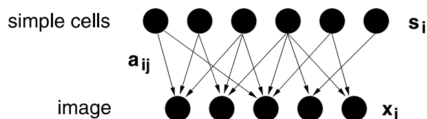
Fig. 1. The linear sparse coding neural network. Units are depicted by filled circles, and arrows represent conditional dependencies (in the generative model) between the units. Upon observing data \mathbf{x} the hidden neuron activities s_i are calculated as the most probable latent variable values to have generated the data. On a longer timescale, the generative weights a_{ij} are adapted to allow typical data to be represented sparsely.
