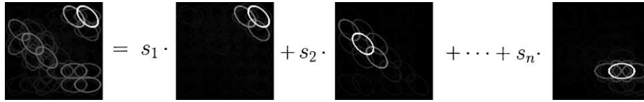
Fig. 6. Sparse coding of complex cell responses. Each complex cell activity pattern is represented as a linear combination of basis patterns \mathbf{a}_i . The goal is to find basis patterns such that the coefficients s_i are as ‘sparse’ as possible, meaning that for most input patterns only a few of them are needed to represent the pattern accurately. Cf. Eq. (2).
