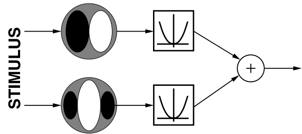
Fig. 4. Complex cell model used. The response of a complex cell was obtained by linearly filtering with quadrature Gabor filters, taking squares, and summing.
