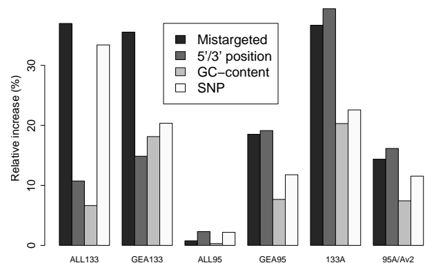
Fig. 3. Increase in the average variance of the probes associated with the investigated noise sources: mistargeted probes having errors in the genomic alignment, most 5'/3' probes of each probe set, GC-rich, and SNP-associated probes. The variances were estimated by RPA and describe the noise level of the probes. The results are shown for the individual ALL and GEA data sets, and for their combined results on both platforms (133A and 95A/Av2).
