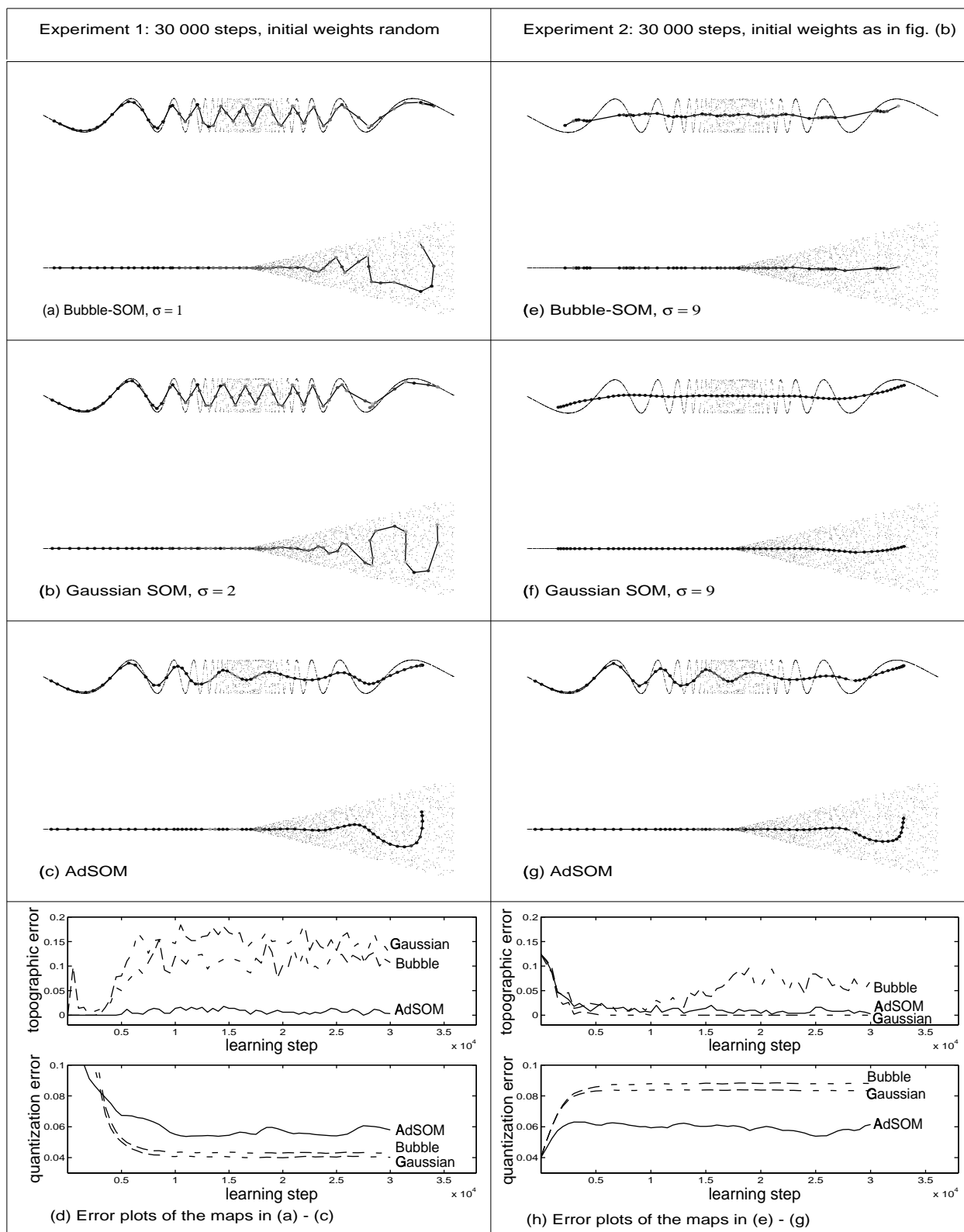
Figure 1. The three-dimensional sample vectors (small dots) with the final positions of the weight vectors superimposed (larger, connected dots), depicted from two different perspectives. The evolution of the topographic and quantization errors during learning is plotted in (d) and (h).
